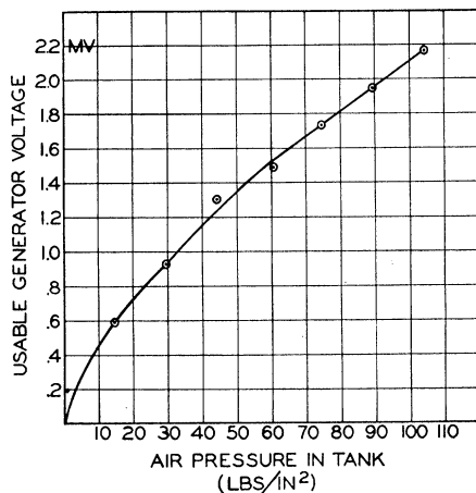
FIG. 1. Curve showing maximum usable generator voltage as a function of air pressure in the enclosing tank. Air pressure is given in lb./in 2 , absolute (not above atmospheric).
