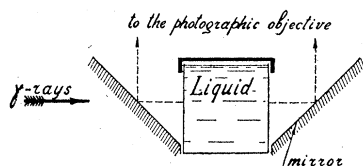
FIG. 1. Arrangement of apparatus.
