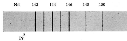
FIG. 1. Mass spectrum of neodymium.
