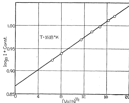
Fig. 2. The Schottky effect.
