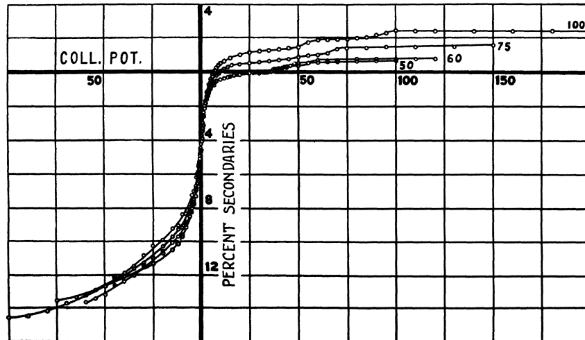
Fig. 4. Curves for accelerating potentials of 50, 60, 75 and 100 volts.
