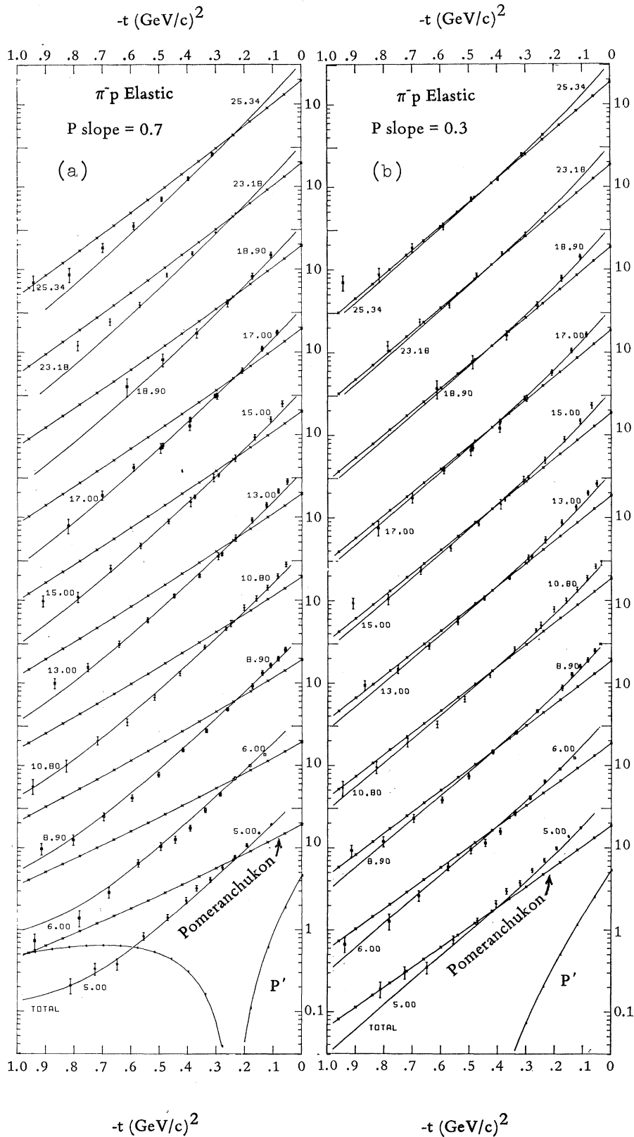
FIG. 2. Fits to \pi^- p elastic d\sigma/dt data, described in Appendix B. The data points for neighboring energy values are separated from each other by one decade. The total ( P+P'+\rho+\rho' ) contribution is presented as an unadorned solid line and that of the P alone as a solid line with \times 's. At the lowest energy, the P' trajectory contribution is given in order to show how its residue zero moves as the P slope is altered. In (a) the P has slope 0.7 and in (b) slope 0.3 (\text{GeV/c})^{-2} .
