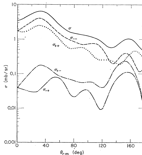
FIG. 18. Microscopic predictions of the partial cross sections [cf. Eq. (1)] for ^{54}\text{Fe} . For these calculations V_0 is -65 MeV and V_1 is -30 MeV. The wave function is assumed to be:
