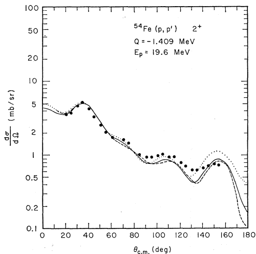
FIG. 15. Collective-model predictions of the differential cross section with the optical parameters of Table II. The curves are identified as in Fig. 13.
