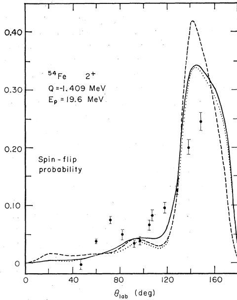
FIG. 3. Spin-flip probability S(\theta) for ^{54}\text{Fe} . The curves are collective-model DWBA predictions with three types of spin-orbit terms: Full Thomas term (solid); U(1) only, Eq. (7a), (dotted); and nondeformed spin-orbit (dashed).
