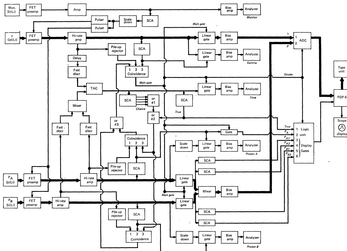
FIG. 1. Simplified block diagram of the electronics. The heavy lines indicate the paths of the analog signals from the two proton counters and the \gamma counter.
