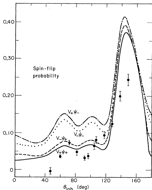
FIG. 17. Microscopic model predictions of S(\theta) for ^{54}\text{Fe} . For these curves V_0 is -65 MeV, V_1 is \pm 30 MeV. The ground state was assumed to be (f_{7/2})_{0^+} . The 2^+ state was assumed to be:
