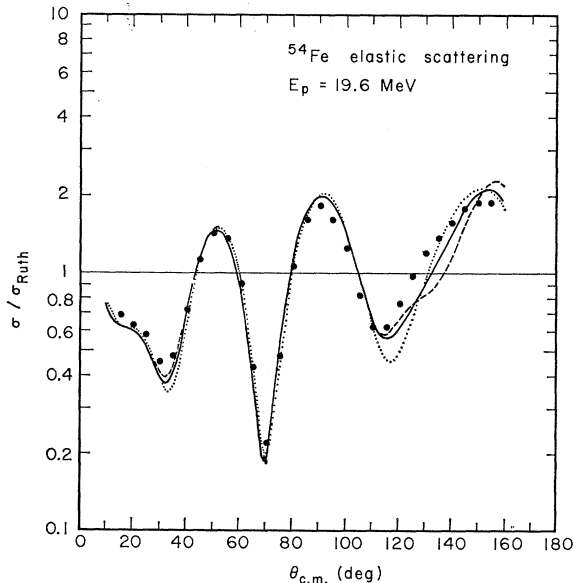
FIG. 9. Ratio of the elastic scattering cross section for ^{54}\text{Fe} to the Rutherford cross section. The solid curve is an optical-model fit using the best-fit parameters of Table I. The dotted and dashed curves are fits using the parameters of Table II with V_{so} fixed at 4 and 6 MeV, respectively.
