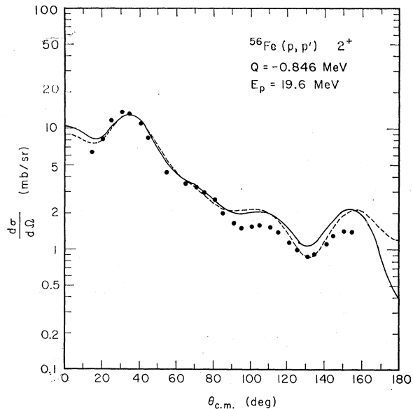
FIG. 8. Differential cross section for ^{56}\text{Fe} . The curves are collective-model DWBA predictions as described for Fig. 3.
