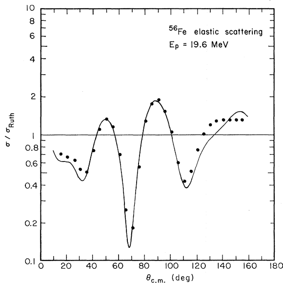
FIG. 11. Ratio of the elastic scattering cross section for ^{56}\text{Fe} to the Rutherford cross section. The curve is an optical-model fit with the parameters of Table I.
