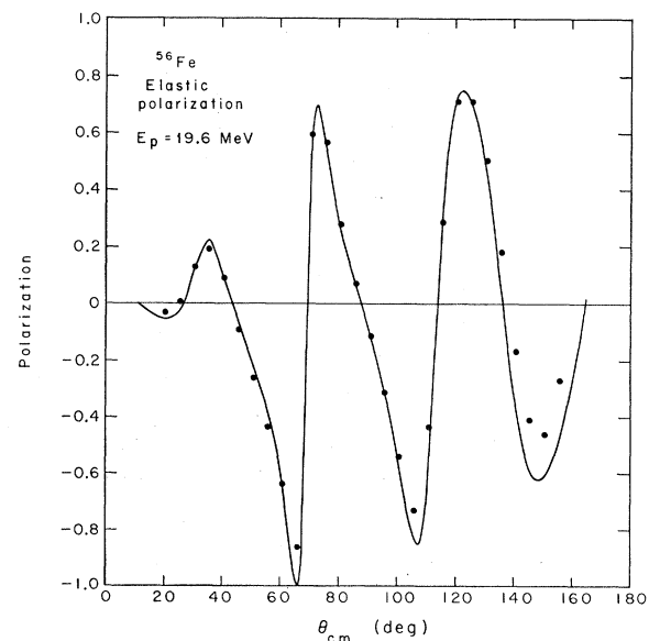
FIG. 12. Polarization in elastic scattering (Ref. 2) from ^{56}\text{Fe} . The curve is an optical-model fit with the parameters of Table I.
