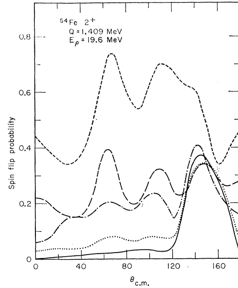
FIG. 16. Microscopic model predictions of S(\theta) for ^{54}\text{Fe} . For all these curves, V_0 = V_1 = -65 MeV. The ground state was assumed to be (f_{7/2})^2_0^+ . The 2^+ state was assumed to be: (f_{7/2})^2_2^+ (solid curve) (f_{7/2}, f_{5/2})^2_2^+ (dashed curve) (f_{7/2}, p_{3/2})^2_2^+ (broken curve), \{0.707 (f_{7/2})^2_2^+ + 0.707 (f_{7/2}, p_{3/2})^2_2^+\} (dotted curve), \{0.707 (f_{7/2})^2_2^+ - 0.707 (f_{7/2}, p_{3/2})^2_2^+\} (dot-dashed curve).
