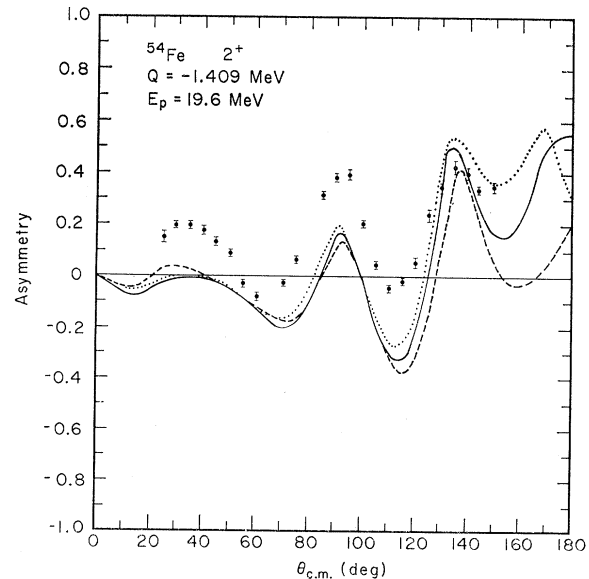
FIG. 14. Collective-model predictions of the asymmetry with the optical parameters of Table II. The curves are identified as in Fig. 13.
