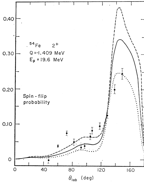
FIG. 13. Collective-model predictions of S(\theta) with the optical parameters of Table II. These were obtained by fixing the spin-orbit well depth at 4 (dotted), 5 (solid), and 6 MeV (dashed).
