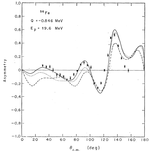
FIG. 6. Asymmetry for ^{56}\text{Fe} , measured at Saclay (Ref. 2). The curves are collective-model DWBA predictions as described for Fig. 3.
