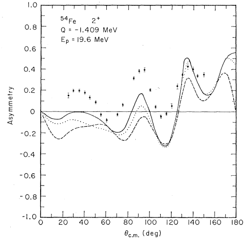
FIG. 5. Asymmetry for ^{54}\text{Fe} , measured at Saclay (Ref. 2). The curves are collective-model DWBA predictions as described for Fig. 3.
