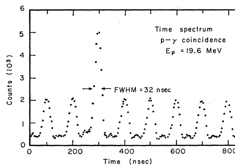
FIG. 2. Pulse-height spectrum from the TAC. The start pulse came from a proton fast discriminator; the stop pulse came from the \gamma fast discriminator. The SCA's were set so that 0.40 < E_\gamma < 3.5 MeV. The large peak is the true peak; the other peaks correspond to chance coincidences.
