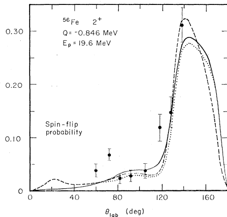
FIG. 4. Spin-flip probability S(\theta) for ^{56}\text{Fe} . The curves are collective-model DWBA predictions as described for Fig. 3.
