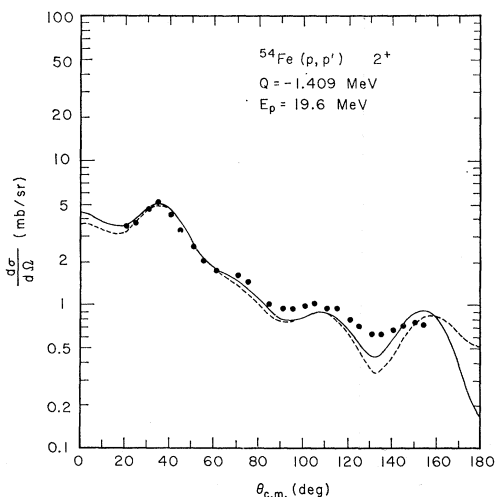
FIG. 7. Differential cross section for ^{54}\text{Fe} . The curves are collective-model DWBA predictions as described for Fig. 3.
