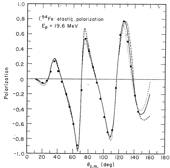
FIG. 10. Polarization in elastic scattering (Ref. 2) from ^{54}\text{Fe} . The curves are optical-model fits with the parameters of Tables I and II. The curves are identified in Fig. 9.
