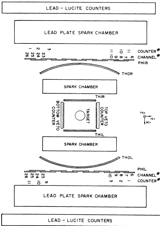
FIG. 3. End view of the detection apparatus.
