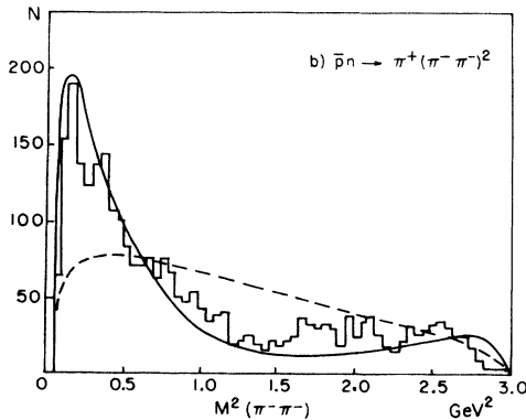
FIG. 1. (a) \pi^+\pi^- and (b) \pi^-\pi^- invariant-mass distributions for the decay \bar{p}n \rightarrow \pi^+\pi^-\pi^- . The continuous curves correspond to the values of c_{nm} stated in the text. The dashed curve in (b) is the phase space.
