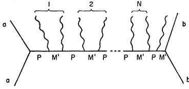
FIG. 5. The most general diagram with a Pomeranchuk trajectory at vertex a and a meson trajectory at vertex b , after contraction of meson trajectories.
