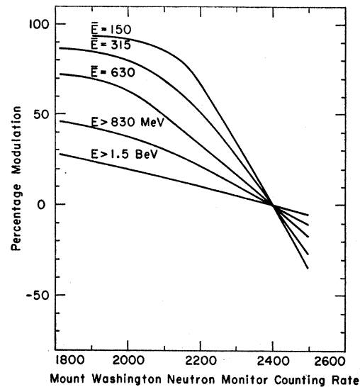
Fig. 4. Modulation of helium nuclei of various energies as a function of Mt. Washington neutron monitor counting rate.
