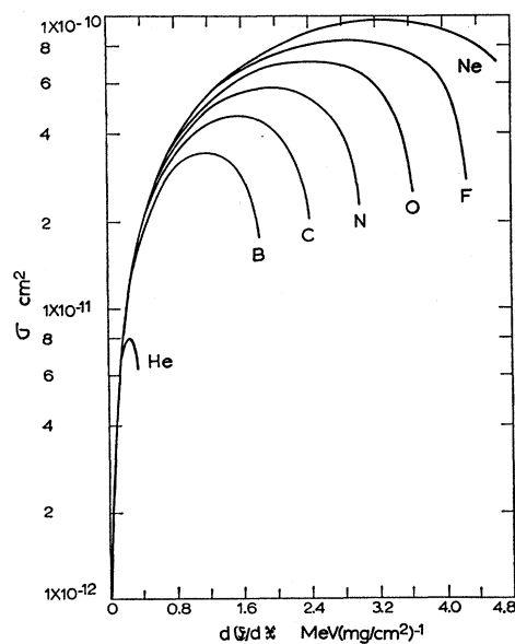
FIG. 5. Theoretical plot of \sigma versus d\mathcal{E}/d\tau .
