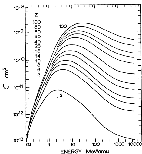
FIG. 3. Theoretical values of the cross section \sigma for activation of a luminescence center in NaI(Tl) versus the ion energy \mathcal{E} , using the point-target approximation, valid for \sigma \geq 3 \times 10^{-11} cm 2 .
