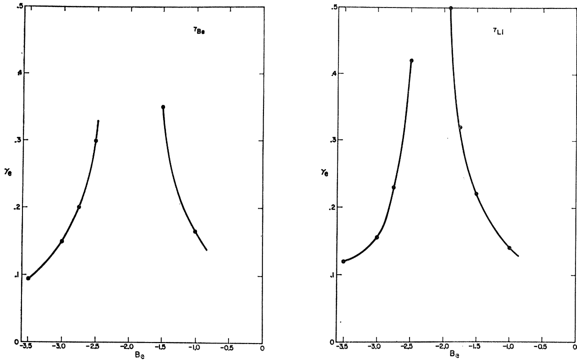
FIG. 19. \text{Li}^7 and \text{Be}^7 boundary value variations showing the value of the elastic reduced-width amplitude for the 4P_{5/2} state in \text{Li}^7 and \text{Be}^7 which gives the best fit for a given value of the boundary value B_e . The lines are smooth curves connecting the calculated points.
