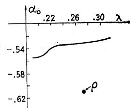
FIG. 8. Curve on which T_0(\frac{4}{3}, \frac{4}{3}) = \frac{5}{2}T_2(\frac{4}{3}, \frac{4}{3}) . The \rho parameters are (-0.61, 0.27) ; the apparent distance from this point (heavy dot in the figure) to the curve is exaggerated by the large scale of this figure.
