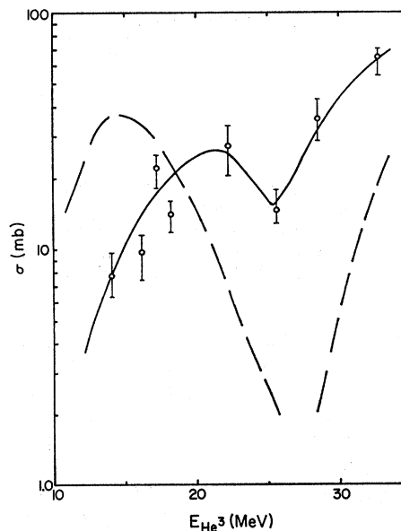
FIG. 2. Excitation function of the (\text{He}^3, \alpha) reaction. The solid curve is drawn through the experimental points. The dashed curve is the result of a statistical-theory calculation.
