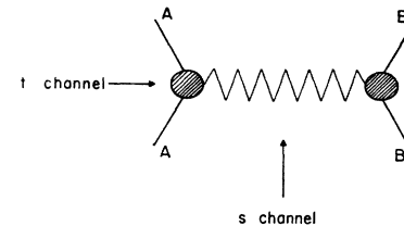
FIG. 1. Meson-exchange model for the elastic-scattering amplitude at high energy.
