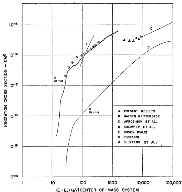
FIG. 2. Total ionization cross section up to 2900-eV lab energy compared with results of other investigators.
