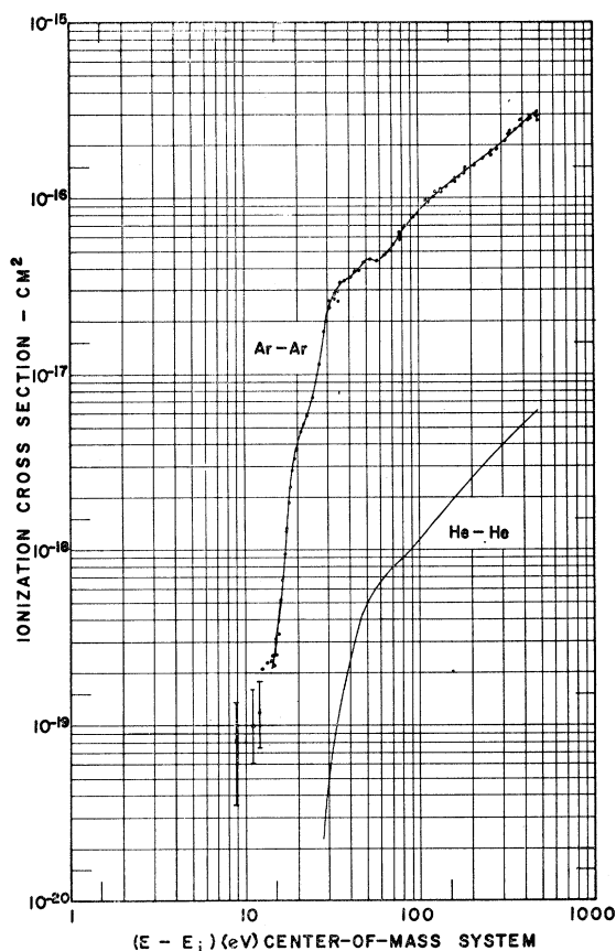
FIG. 1. Total ionization cross section \sigma_{-} for Ar-Ar collisions as a function of excess c.m. energy. E_i is the ionization potential.
