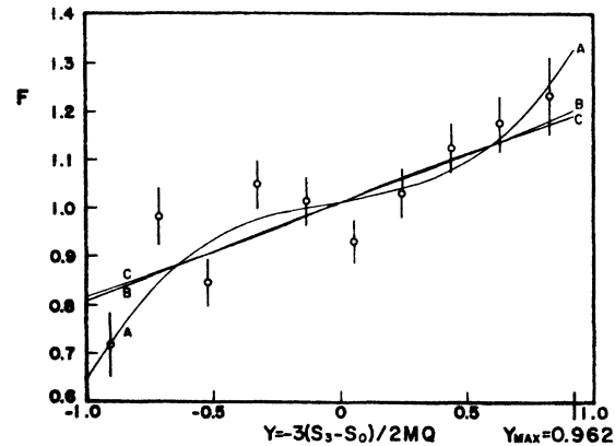
FIG. 8. Energy dependence of the reduced \pi^- energy spectrum for the Mitra and Ray model for \tau decay. Curve A is for the best-fit parameters, M_r = 335 MeV and \Gamma_r = 65 MeV. Curve B is for the parameters M_r = 400 MeV and \Gamma_r = 210 MeV, curve C is for M_r = 475 MeV and \Gamma_r = 10 MeV. Curves A, B, and C correspond to points A, B, and C on Fig. 7.
