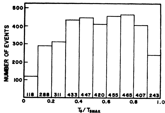
FIG. 1. Histogram of the \pi^- energy distribution for 3587 \tau^+ decays. The number of events in each division is indicated.
