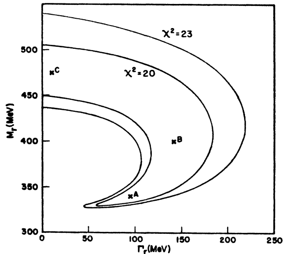
FIG. 5. Contour plot of constant \chi^2 for the mass M_r and full width \Gamma_r of the resonance in the Brown and Singer model for \tau decay. Point A corresponds to the best-fit parameters, \chi^2=16.1 ; the points A, B, and C correspond to curves A, B, and C in Fig. 6. The lines \chi^2=20 and \chi^2=23 correspond roughly to one and two standard deviations from minimum \chi^2 , respectively, the "allowed" range for the parameters.
