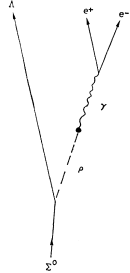
FIG. 6. Diagram for \Sigma^0 \rightarrow \Lambda e^+ e^- .
