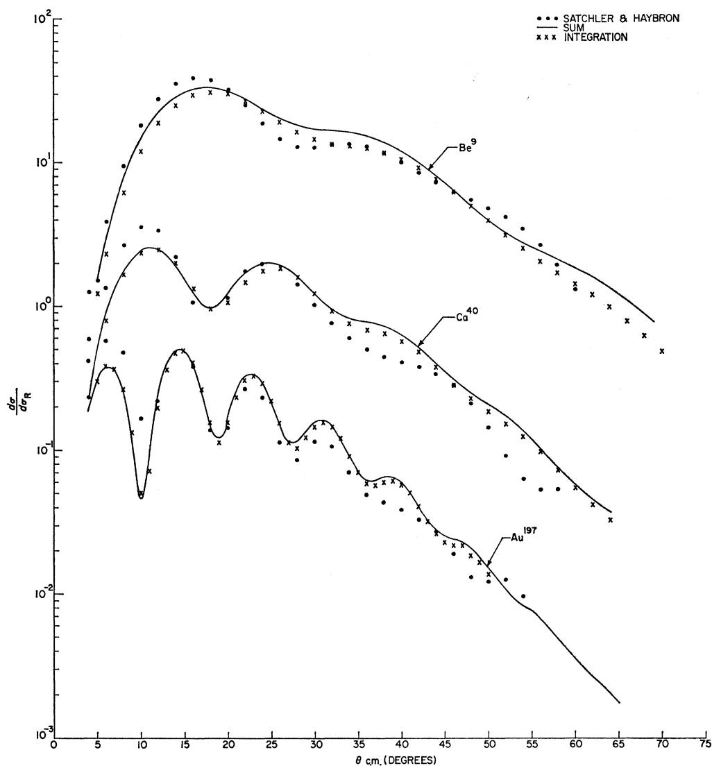
FIG. 4. A comparison of the Frahn-Venter calculation with their modified parameters using a summation (—); the integration (×) those authors use; and optical-model calculations (●) at 182 MeV. The reaction cross section calculated by the summation differs by less than 1% from that calculated by the integration.
