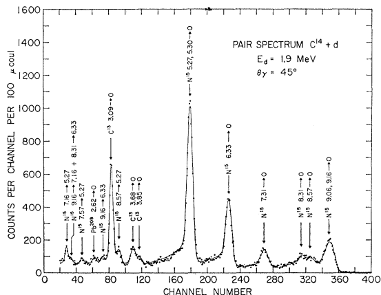
FIG. 3. Gamma-ray pulse-height spectrum measured with a three-crystal pair spectrometer following bombardment of a C 14 target with 1.9-MeV deuterons. The transitions identified all arise from C 14 + d or C 13 + d except the 2.62-MeV peak which arises primarily from inelastic scattering of neutrons in the lead shielding of the pair spectrometer. The solid curve through the experimental points is the result of a computer fit employed to determine gamma-ray intensities.
