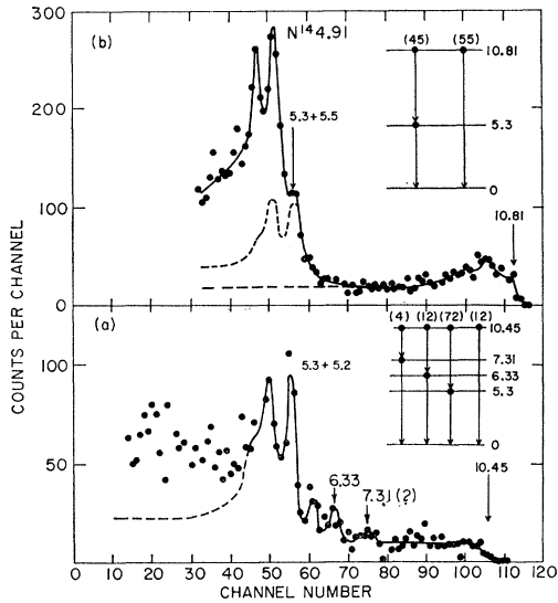
FIG. 10. Gamma-ray spectrum from C^{12,13}+He^3 at \theta_\gamma=90^\circ and E_{He^3}=3.0 MeV in coincidence with the proton groups feeding (a) the N^{15} 10.45-MeV level and (b) the N^{15} 10.81-MeV level and the N^{14} 4.91-MeV level. Gamma-ray peak energies are given in MeV. The decay schemes inferred from the spectra are indicated in the inserts.
