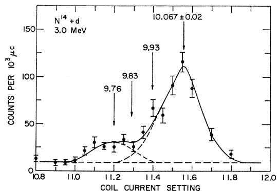
FIG. 21. Partial spectrum of internal-pair lines from levels of N^{15} populated by 3.0-MeV deuteron bombardment of a N^{14} target, indicating the presence of the transitions 9.76 \rightarrow 0 and 10.07 \rightarrow 0 and the expected positions of the 9.83 \rightarrow 0 and 9.93 \rightarrow 0 transitions. The energy calibration was made relative to the 9.052 \rightarrow 0 transition of N^{15} .
