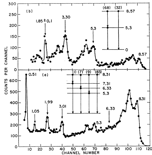
FIG. 11. Gamma-ray spectra from N^{14}(d, p\gamma)N^{15} at \theta_\gamma=90^\circ and E_d=3.0 MeV in coincidence with the proton groups feeding (a) the 8.31-MeV level and (b) the 8.57-MeV level. The gamma-ray peak at 1.85 \pm 0.1 MeV in (b) is presumed to arise from a contaminant reaction. The decay schemes inferred from the spectra are indicated in the inserts. Gamma-ray peak energies are given in MeV.
