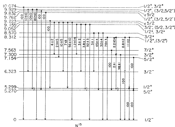
FIG. 24. Level scheme of N^{15} showing spins, parities and decay modes of the bound levels. The various assignments and branching ratios are obtained as a synthesis of the results of this experiment with those reported from other sources, as explained in the text. Uncertain or less likely assignments are enclosed in parentheses.
