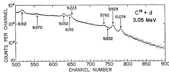
FIG. 18. Partial Li-Ge two-escape peak gamma-ray spectra from C^{14}(d,n\gamma)N^{15} at E_d=3.05 MeV and \theta_\gamma=90^\circ . The resolution of the detector for the two-escape peaks is about 11 keV and the dispersion is about 7 keV/channel. The peaks correspond to ground-state transitions in N^{15} and are labeled by the excitation energies (in MeV) of the initial states (following Table VII). The important information obtained from this spectrum is the relative intensities of the various lines and the fact that all the observed lines are Doppler broadened.
