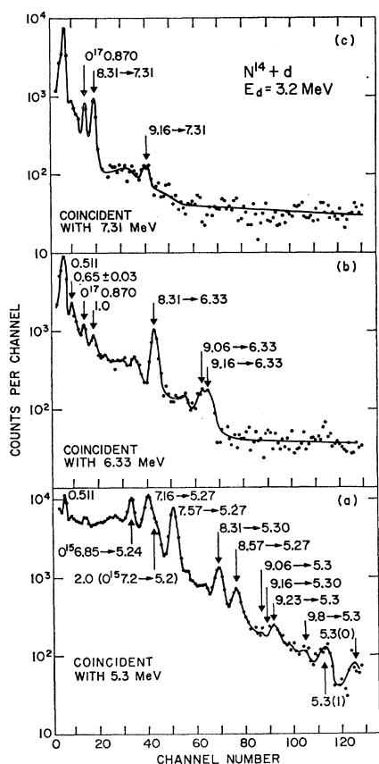
FIG. 14. Gamma-gamma coincidence spectra from N^{14}+d at E_d=3.2 MeV. The spectra show the low-energy ( E_\gamma < 5.4 MeV) gamma rays in coincidence with the ground-state decays of (a) the N^{15} , O^{15} 5-MeV levels, (b) the N^{15} 6.33-MeV level and O^{15} 6.16-MeV level, and (c) the N^{15} 7.31-MeV level. Cascade transitions in N^{15} are labeled by the energies of the initial and final levels (in MeV) between which the transitions occur. Two O^{15} cascade transitions are also labeled in (a). The origin of the 0.511-, 0.870-, and 1.0-MeV peaks is the same as for Fig. 13. The origin of the peak at 0.65 \pm 0.03 MeV is unknown.
