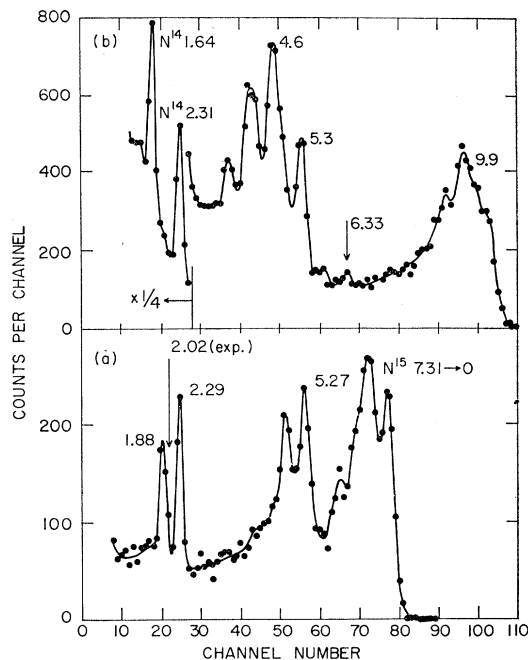
FIG. 8. Gamma-ray spectra from C^{12,13}+He^3 at \theta_\gamma = 90^\circ and E_{He^3} = 3.0 MeV in coincidence with the proton groups feeding (a) the N^{15} 7.16-, 7.31-, and 7.57-MeV triplet and (b) the N^{15} 9.77-, 9.83-, 9.94-, and 10.06-MeV quadruplet and the N^{14} 3.95-MeV level. Gamma-ray peak energies are given in MeV.
