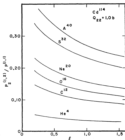
FIG. 2. The ratio \lambda D_{21} = P_2^{(1,2)}/P_1^{(1,1)} plotted as a function of the adiabaticity parameter \xi for heavy ions bombarding Cd^{114} at \theta = 180^\circ with Q_{22} = 1 b.
