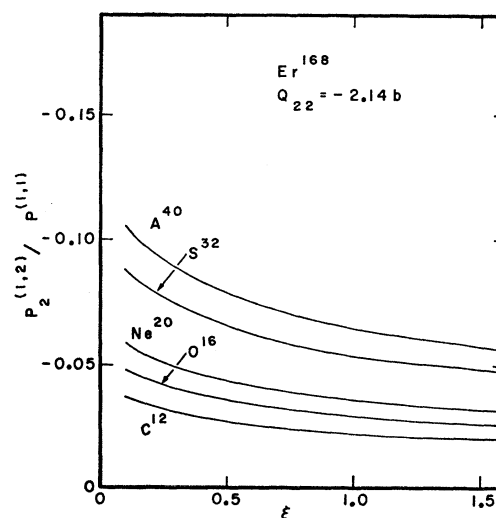
FIG. 4. The ratio \lambda D_{21} = P_2^{(1,2)}/P_1^{(1,1)} plotted as a function of the adiabaticity parameter \xi for heavy ions bombarding Er^{168} at \theta = 180^\circ with Q_{22} = -2.14 b.
