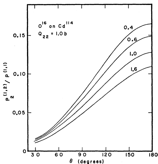
FIG. 1. The ratio \lambda D_{21} of the second-order reorientation effect P_2^{(1,2)} to the first-order probability P_1^{(1,1)} plotted as a function of the scattering angle in the center-of-mass system \theta for O^{16} bombarding Cd^{114} . The curves are designated by several fixed values of the adiabaticity parameter \xi and Q_{22} , the static quadrupole moment of the lowest 2^+ state, is taken as 1 b.
