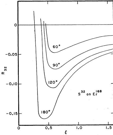
FIG. 5. The ratio R_{32} = [P^{(1,3)} + P^{(2,2)}]/P^{(1,2)} plotted as a function of \xi for S^{32} bombarding Er^{168} at several scattering angles in the center-of-mass system with Q_{22} = -2.14 b.
