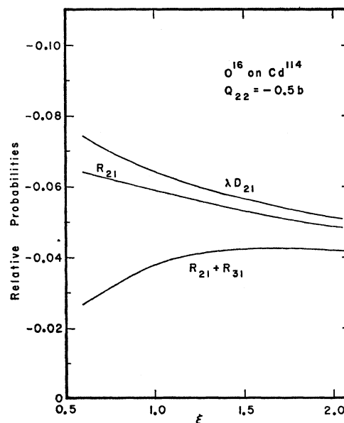
FIG. 7. The quantities \lambda D_{21} = P^{(1,2)}/P^{(1,1)} , R_{21} = P^{(1,2)}/P^{(1,1)} , and (R_{21} + R_{31}) = [P^{(1,2)} + P^{(2,2)} + P^{(1,3)}]/P^{(1,1)} plotted as a function of \xi for O^{16} on Cd^{114} at \theta = 180^\circ with Q_{22} = -0.5 b.
