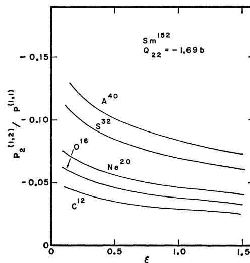
FIG. 3. The ratio \lambda D_{21} = P_2^{(1,2)}/P_1^{(1,1)} plotted as a function of the adiabaticity parameter \xi for heavy ions bombarding Sm^{152} at \theta = 180^\circ with Q_{22} = -1.69 b.
