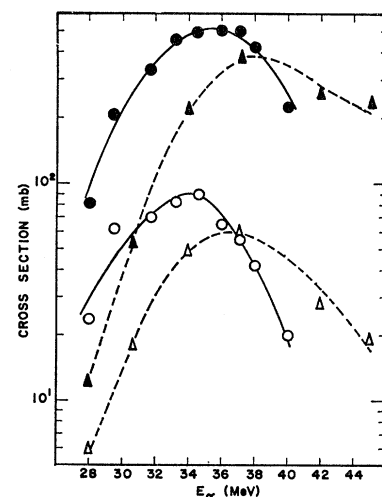
FIG. 7. Excitation functions for ^{137m}\text{Ce} (filled symbols) and ^{137g}\text{Ce} (open symbols) in the reaction ^{136}\text{Ba}(\alpha, 3n) . The circles are the results from this work and the triangles are data taken from Ref. 9. Bombarding energy is in the laboratory system.
