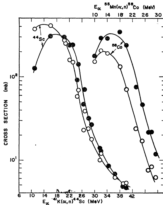
Fig. 5. Excitation functions for the reactions ^{41}\text{K}(\alpha, n) and ^{55}\text{Mn}(\alpha, n) . Open circles denote the ground-state nuclide and filled circles the metastable nuclide. Bombarding energy is in the laboratory system. The lower energy scale is for the ^{41}\text{K}(\alpha, n) reaction and the upper scale for the ^{55}\text{Mn}(\alpha, n) reaction.
