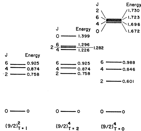
FIG. 3. Excitation spectrum for (9/2)^2 and (9/2)^4 configurations with delta interaction. Only the lowest two J=0, 2, 4 , and 6 states are shown. Energies are expressed in units of the (9/2)^2 ground state energy and the scale is shifted so that the ground state is at 0.
