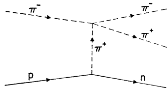
FIG. 8. Diagram for one-pion exchange (OPE).
