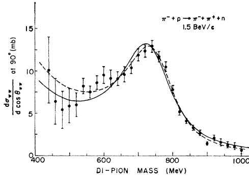
FIG. 9. \partial\sigma_{\pi\pi}/\partial \cos\theta_{\pi\pi} , averaged over the interval -0.2 < \cos\theta_{\pi\pi} < 0.2 . The curves show fits obtained with a Breit-Wigner resonance plus a background term varying as \lambda^2 . Solid curve: no resonant-nonresonant interference term, m_0 = 736 MeV, \Gamma = 176 MeV, 1.5% \chi^2 probability. Dashed curve: with interference term, m_0 = 753 MeV, \Gamma = 170 MeV, 47% \chi^2 probability. Both fits show an 11 mb resonant contribution to the cross section.
