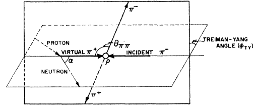
FIG. 11. Illustration of the Treiman-Yang angle in the dipion rest frame.
