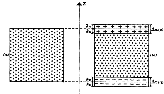
FIG. 2. Separation of the two-photon helicity states in the limiting case of total reflection. Cross sections of: left, incoming beam, right, outgoing beam; ( a ) any polarization state, ( p ) positive helicity, ( n ) negative helicity.
