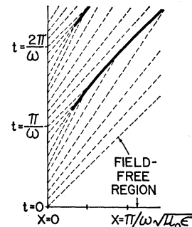
FIG. 1. Space-time evolution of the electromagnetic radiation field for Case 1 with \hat{E}^2 = \epsilon/\eta . Dashed lines represent the E = \text{constant} characteristics while heavy solid lines represent the electromagnetic shocks.
