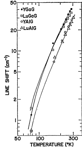
FIG. 3. Shift of the lower-energy R line below its position at 4.2°K for the four garnets. The curves are calculated from Eq. (4).
