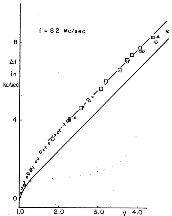
FIG. 4. Results of the passive method. The \odot , \times , \triangle , \square , represent the results of four runs. The lower curve is obtained by correcting the experimental data for effects of the superconducting coil in the tank circuit.
