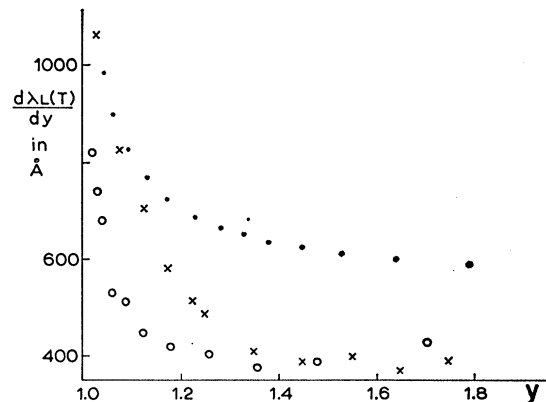
FIG. 6. d\lambda_L(T)/dy as a function of y for the present results, for the results of Dobbs and Perz (DP), and for the BCS theory. All curves are based on \lambda_L(0) = 390 \text{ \AA} .
