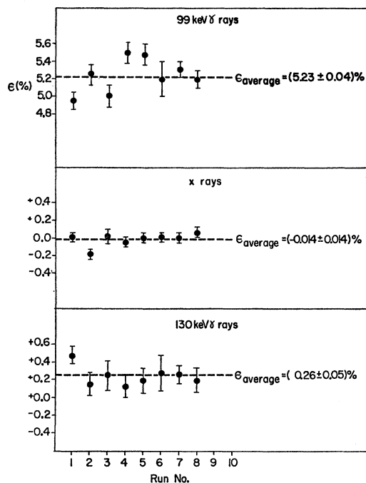
FIG. 6. Plot of the magnitude of the Mössbauer effect [N(65^\circ\text{K}) - N(20^\circ\text{K})]/N(65^\circ\text{K}) for the x rays and the 99- and 130-keV gamma rays, measured in consecutive runs of approximately 4 h each.
