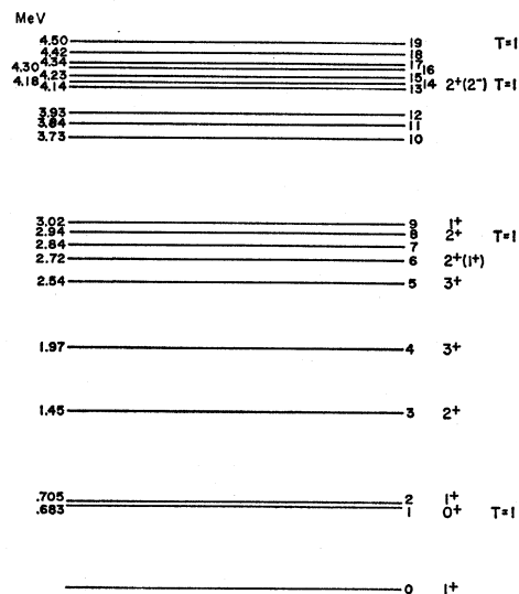
Fig. 3. The lower energy levels in P^{30} . T values are isotopic spins; spin parities in parentheses are less likely alternatives.
