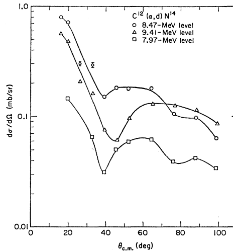
FIG. 8. Angular distributions of deuterons from formation of the 7.97-, 8.47-, and 9.41-MeV levels of N 14 .
