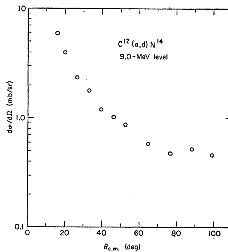
FIG. 9. Angular distribution of deuterons from formation of the 9.00-MeV level of N 14 .
