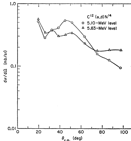
FIG. 6. Angular distributions of deuterons from formation of the 5.10- and 5.83-MeV levels of N^{14} . Small contributions from the 4.91- and 5.69-MeV levels, respectively, are included.
