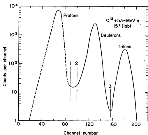
FIG. 2. Particle identifier spectrum at a scattering angle of 15 deg (lab) from bombardment of C 12 with 53-MeV alpha particles. The discriminator settings are represented by lines 1, 2, and 3.
