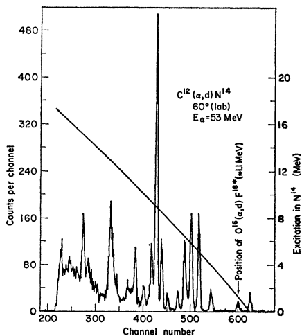
FIG. 4. Deuteron energy spectrum from the C^{12}(\alpha,d)N^{14} reaction at 60^\circ (lab).
