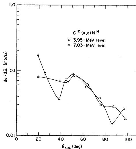
FIG. 7. Angular distributions of deuterons from formation of the 3.95- and 7.03-MeV levels of N^{14} .
