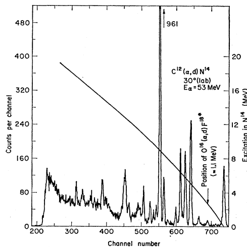
FIG. 3. Deuteron energy spectrum from the C 12 ( \alpha, d )N 14 reaction at 30°(lab).
