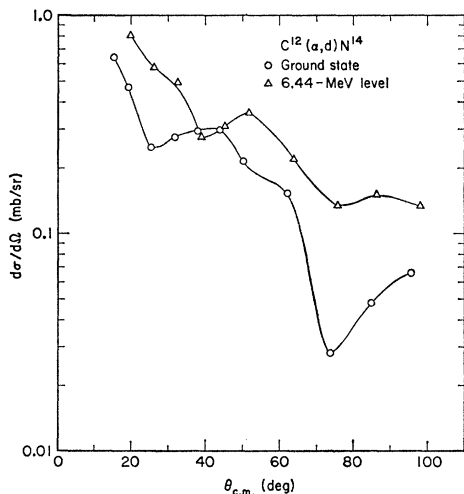
FIG. 5. Angular distributions of deuterons from formation of the ground state and 6.44-MeV levels of N^{14} . The latter includes a small contribution from the 6.23-MeV level.
