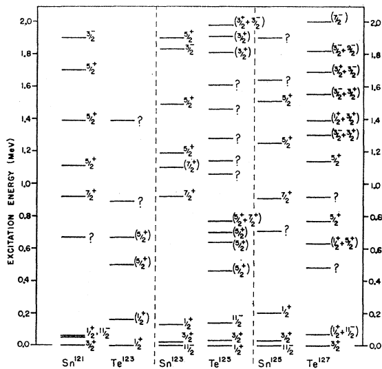
Fig. 13. A comparison of the detailed neutron energy spectra in the isotonic pairs Sn 121 , Te 123 ; Sn 123 , Te 126 ; and Sn 125 , Te 127 .
