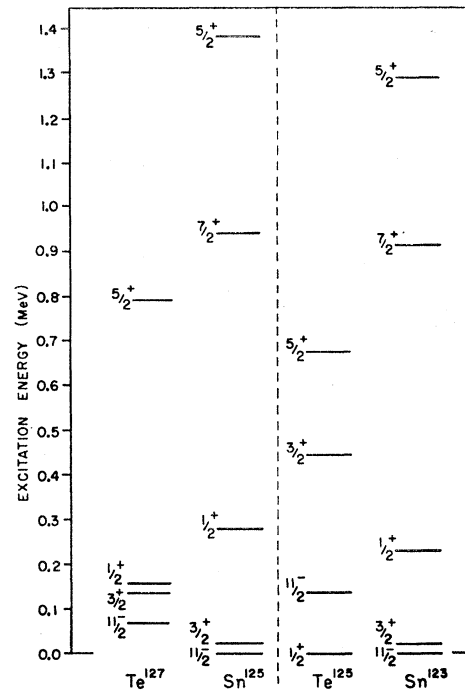
Fig. 14. A comparison of the single-quasiparticle neutron energy spectra in the isotonic pairs Sn 128 , Te 125 and Sn 126 , Te 127 .
