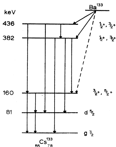
FIG. 2. Disintegration scheme of \text{Ba}^{133} as indicated by present results combined with those of the references of this paper.
