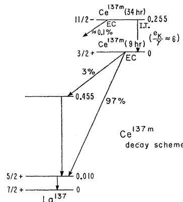
FIG. 3. Existing decay scheme for Ce^{137m} .
