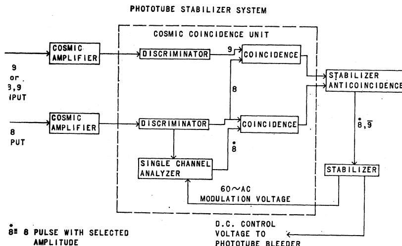
FIG. 3. Schematic diagram of stabilizer circuit.
