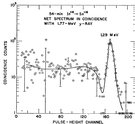
Fig. 3. Spectrum in coincidence with the 1.77-MeV gamma ray. The coincidences due to the underlying Compton distribution of the 2.12-MeV gamma ray have been subtracted.
