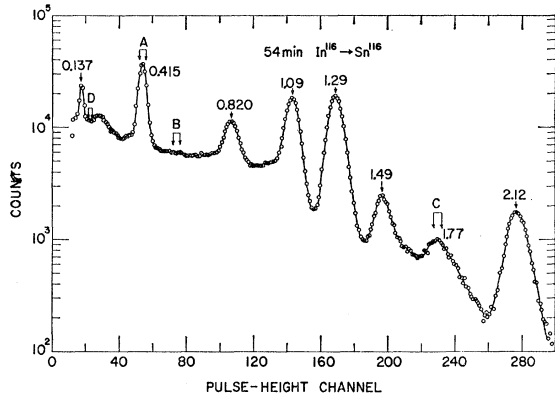
Fig. 1. NaI(Tl) (3×3 in.) pulse-height spectrum of \gamma rays in \text{Sn}^{116} following the decay of 54-min \text{In}^{116} .
