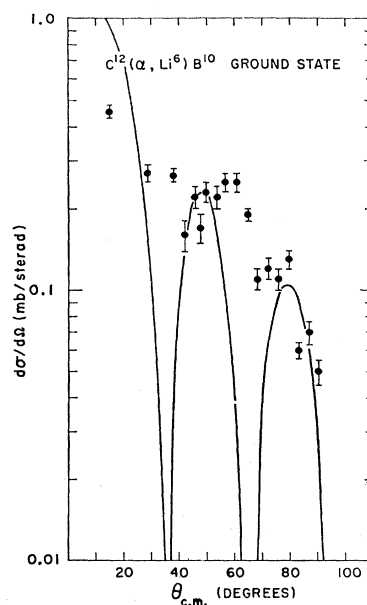
FIG. 10. Angular distribution of Li ions from \text{C}^{12}(\alpha, \text{Li}^6)\text{B}^{10} (ground state). The solid curve is expression (1) with L=2 and R_0=5.4 F .
