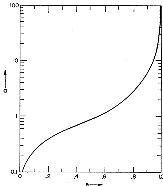
FIG. 1. The semimajor axis a as a function of the eccentricity e in the decay of a two-point mass system. Here, c_0 is chosen to be 1.
