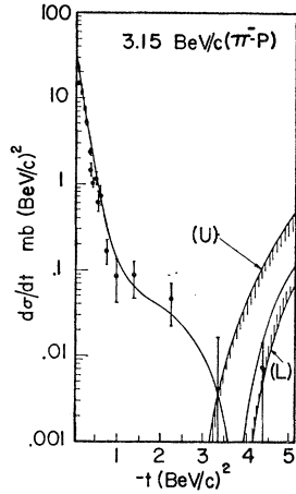
FIG. 2. Differential cross sections for elastic \pi^- - p scattering at 3.15 BeV/c. The curves (U) and (L) show, respectively, the upper and lower limit for the d\sigma/dt in the backward direction. The solid curve shows our results obtained from the expression |d\sigma/dt| = [\exp\frac{1}{2}(A_0 + A_1 t) + C - \exp\frac{1}{2}\{B_0 + B_1(u - u_0)\}]^2 mb/(BeV/c) 2 with the following values of the parameters: A_0 = 3.7 , A_1 = 7.79 (BeV/c) -2 , C = 0.3 , B_0 = -0.84 and B_1 = 1.14 (BeV/c) -2 . The experimental data are from the work of Perl et al. (Ref. 3).
