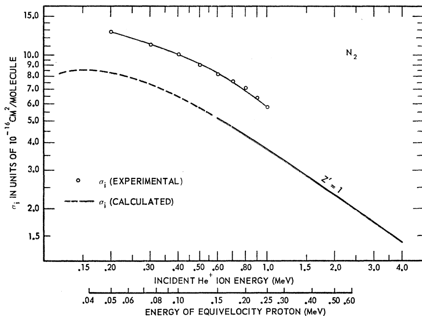
FIG. 4. Apparent ionization cross sections \sigma_i for He + ions incident on molecular nitrogen. Values derived from experimental measurements for incident He + ions are shown for comparison with the calculated curve of \sigma_i = [A(Z')^2 M/E] \ln(BE/M) with A and B evaluated from corresponding proton data (Ref. 8) for Z'=1 .
