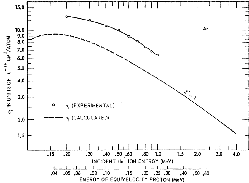
FIG. 3. Apparent ionization cross sections, \sigma_i , for He + ions incident on argon. Values derived from experimental measurements for incident He + ions are shown for comparison with the calculated curve of \sigma_i = [A(Z')^2 M/E] \ln(BE/M) with A and B evaluated from corresponding proton data (Ref. 8) for Z'=1 .
