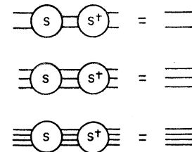
FIG. 1. The unitarity equations for certain S -matrix elements valid just above their physical thresholds. At higher energies the number of intermediate states included depends upon the energy. Equations with S and S † interchanged also hold.
