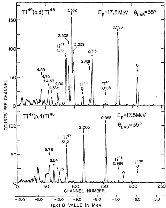
FIG. 2. Energy spectra of the deuterons from the reactions Ti 49 (p,d)Ti 48 and Ti 47 (p,d)Ti 46 at a laboratory angle of 35°, using 17.5-MeV protons.
