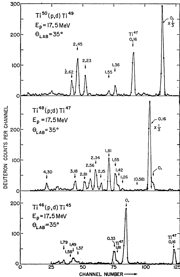
FIG. 1. Energy spectra of the deuterons from the reactions Ti 50 (p,d)Ti 49 , Ti 48 (p,d)Ti 47 , Ti 46 (p,d)Ti 45 at a laboratory angle of 35°, using 17.5-MeV protons.
