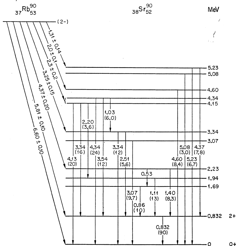
FIG. 9. Partial decay scheme proposed for \text{Rb}^{90} . All energies are in MeV. Relative intensities based on the single-crystal and coincidence data are given in parentheses beneath the gamma-ray energies.
