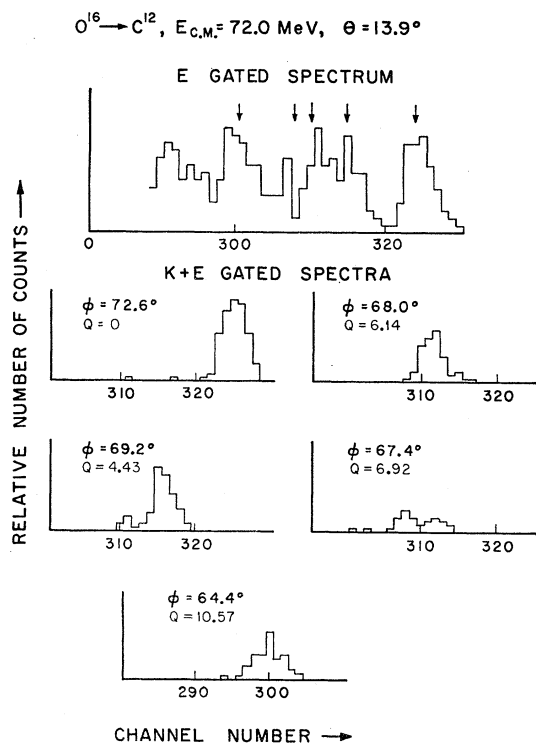
FIG. 6. Typical spectra showing separation of reactions with kinematic coincidence. Scattered-particle spectra are observed at 13.9^\circ in the laboratory for various recoil angles.
