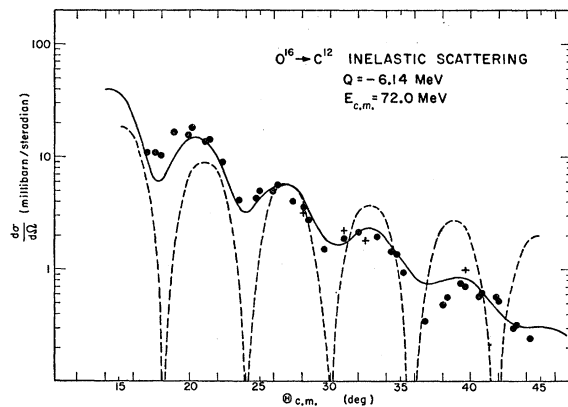
FIG. 10. Comparison of the measured inelastic differential cross section for the excitation of the 6.14-MeV level in O^{16} to the DWBA prediction (solid curve) and to the plane-wave Born approximation prediction (dashed curve). Data points shown as crosses indicate kinematic coincidence techniques used.
