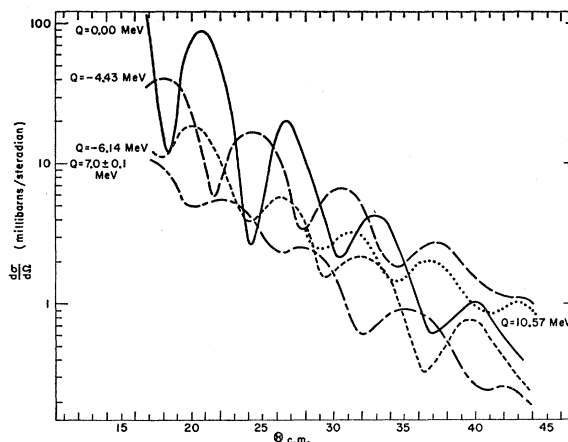
Fig. 7. Measured differential cross sections versus center-of-mass angle for the scattering of 168-MeV O^{16} ions from C^{12} .
