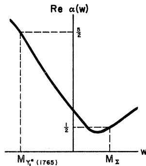
FIG. 6. A possible connection between the trajectories of \Sigma and 1765-MeV Y_1^* .
