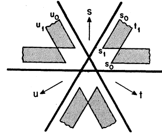
FIG. 2. Regions where Regge terms dominate the double-spectral functions.
