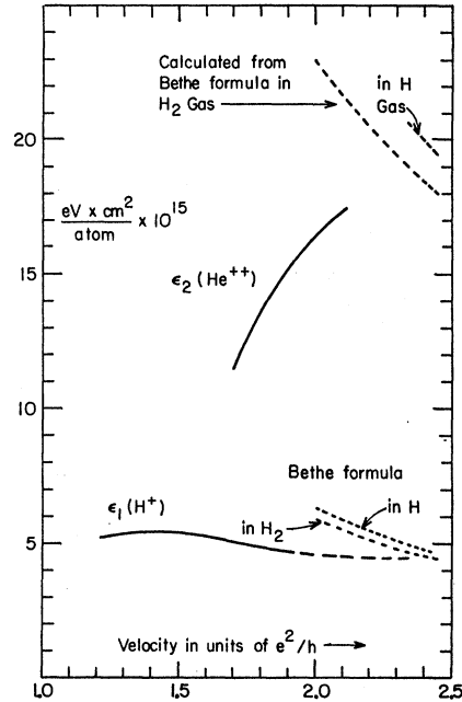
FIG. 6. Experimental partial stopping powers of H_2 gas for protons and for alpha particles. Dashed curves are calculated values using Bethe's equation (Table VII) with 1.105 Rk \equiv I = 15 for H gas and I = 19 for H_2 gas.
