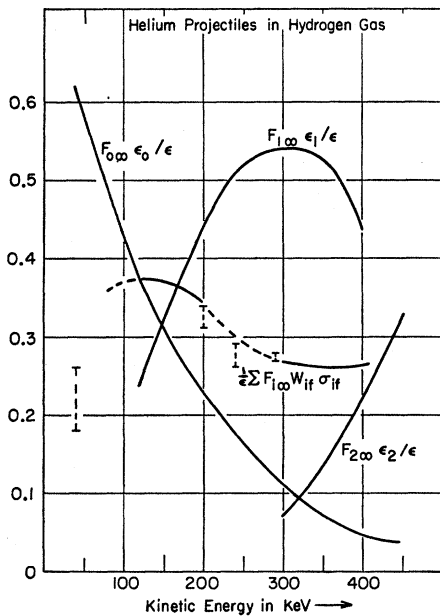
FIG. 5. The fraction of the total stopping power attributable to \text{He}^0 , excepting electron-loss collisions; to \text{He}^+ , excepting capture or loss; and to \text{He}^{++} excepting capture. [\sum F_{i\infty} W_{if} \sigma_{if}] / \epsilon is the fractional loss in collisions involving change of charge of the projectile.
