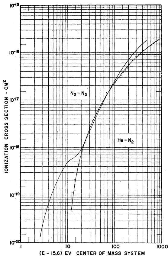
FIG. 6. He-N 2 ionization cross section.
