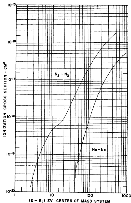
FIG. 5. He-Ne ionization cross section.
