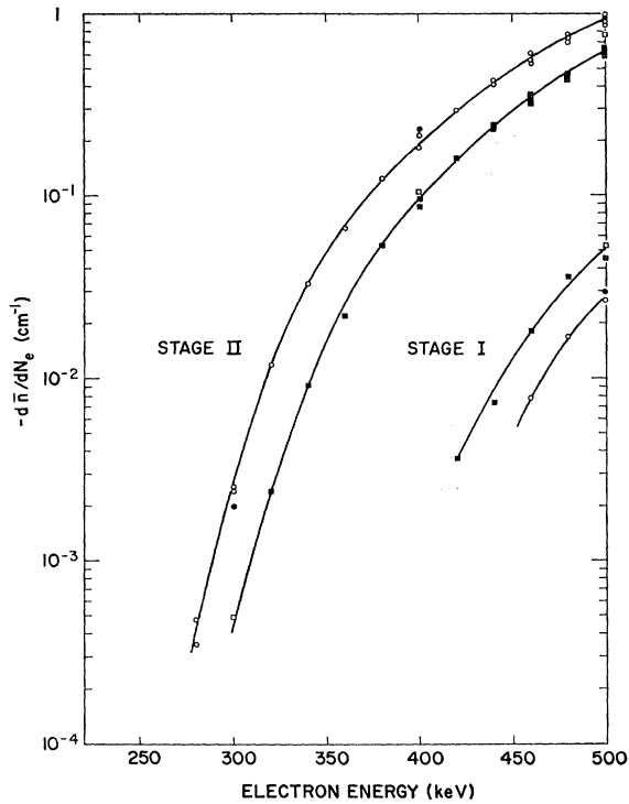
FIG. 2. Carrier removal rate, -d\bar{n}/dN_e , for (111)- and (\bar{1}\bar{1}\bar{1}) -oriented samples, separated into the portion which recovers in stage I and that which recovers in stage II, versus bombarding electron energy. Circles represent data obtained when irradiating the (111) surface and squares are for the (\bar{1}\bar{1}\bar{1}) surface. Filled symbols are for sample 1 and the empty symbols are for sample 2.
