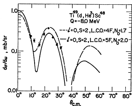
FIG. 14. Angular distribution for the \text{Ti}^{49}(\text{d}, \text{He}^3)\text{Sc}^{48} reaction to the state near 2.1 MeV.
