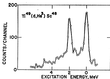
FIG. 13. Spectrum of the \text{Ti}^{49}(\text{d}, \text{He}^3)\text{Sc}^{48} reaction at 20^\circ lab.
