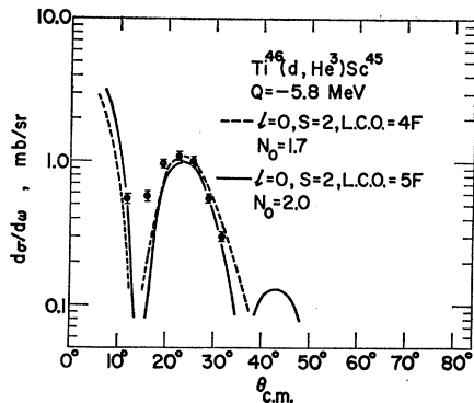
FIG. 6. Angular distribution for the Ti^{46}(d, He^3)Sc^{45} reaction to the 0.92-MeV state.
