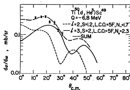
FIG. 16. Angular distribution for the ground-state transition of the \text{Ti}^{50}(\text{d}, \text{He}^3)\text{Sc}^{49} reaction.
