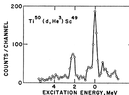
FIG. 15. Spectrum of the \text{Ti}^{50}(\text{d}, \text{He}^3)\text{Sc}^{49} reaction.
