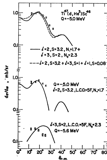
FIG. 8. Angular distributions of the He^3 groups from Ti^{47}(d, He^3)Sc^{46} reaction to the 0.135-MeV and 0.59-MeV states and of the sum of these groups.
