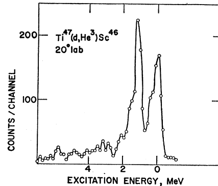
FIG. 7. Spectrum for the Ti^{47}(d, He^3)Sc^{46} reaction at 20^\circ lab.
